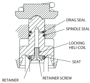
F84L-8 SEAT/RETAINER DETAIL
