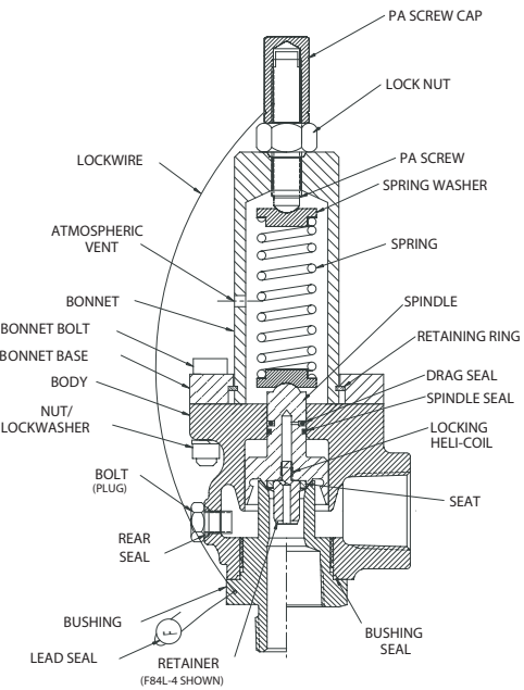
F84L-4/-8 "LARGE" BODY
