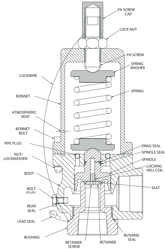
F84L-G/-J "LARGE" BODY
