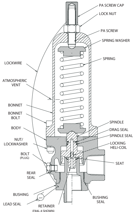
F84L-4/-8 "X-LARGE" BODY
