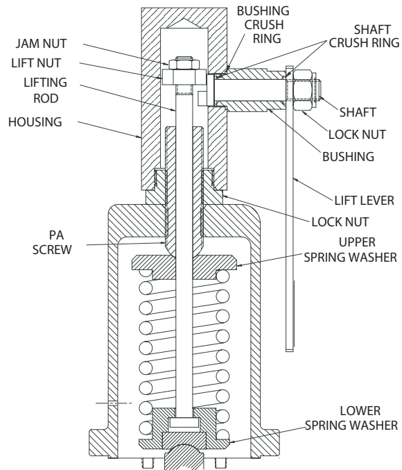
F84L LIFT LEVER ASSEMBLY
