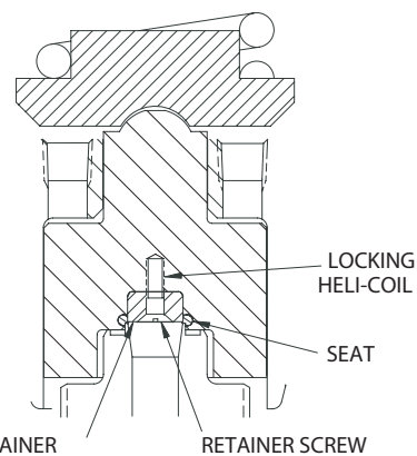
SPINDLE/SEAT DETAIL (NEWER MODELS ONLY)
