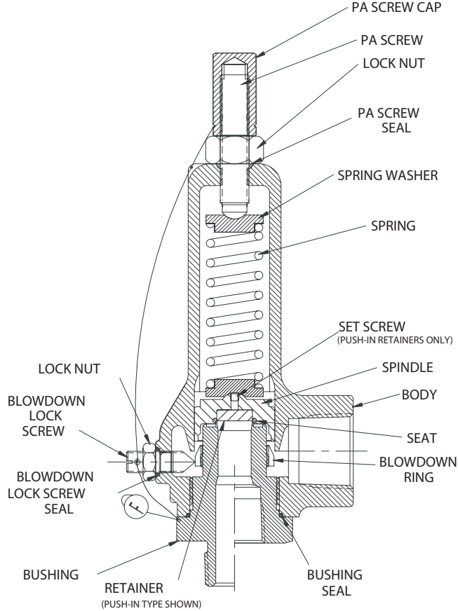
F85-4/6/8 "B" BODY
