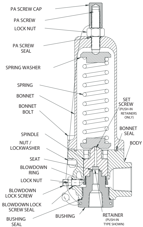
F85-4/6/8 "C" BODY F85-F/G "D" BODY F85-H/J "E" BODY
