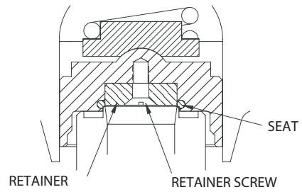
SPINDLE/SEAT DETAIL (NEWER MODELS ONLY)
