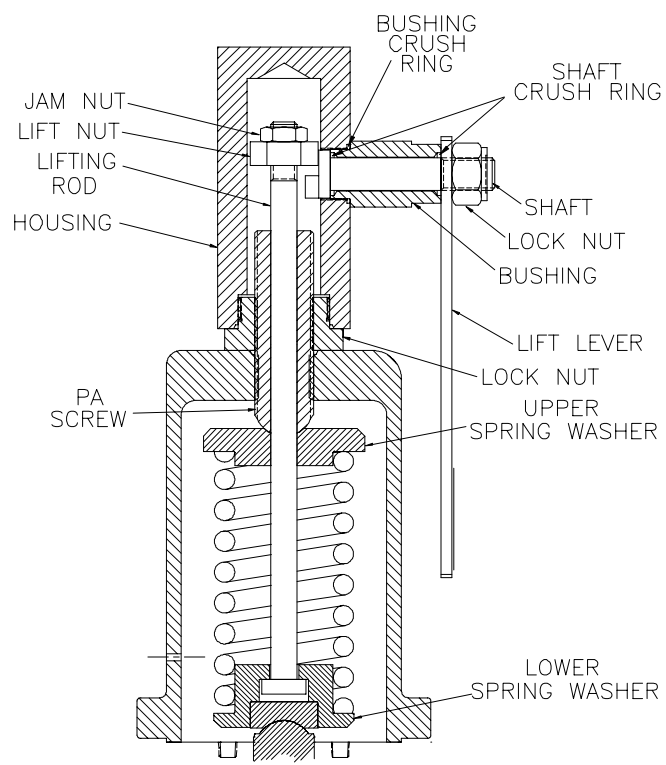
LIFT LEVER ASSEMBLY
